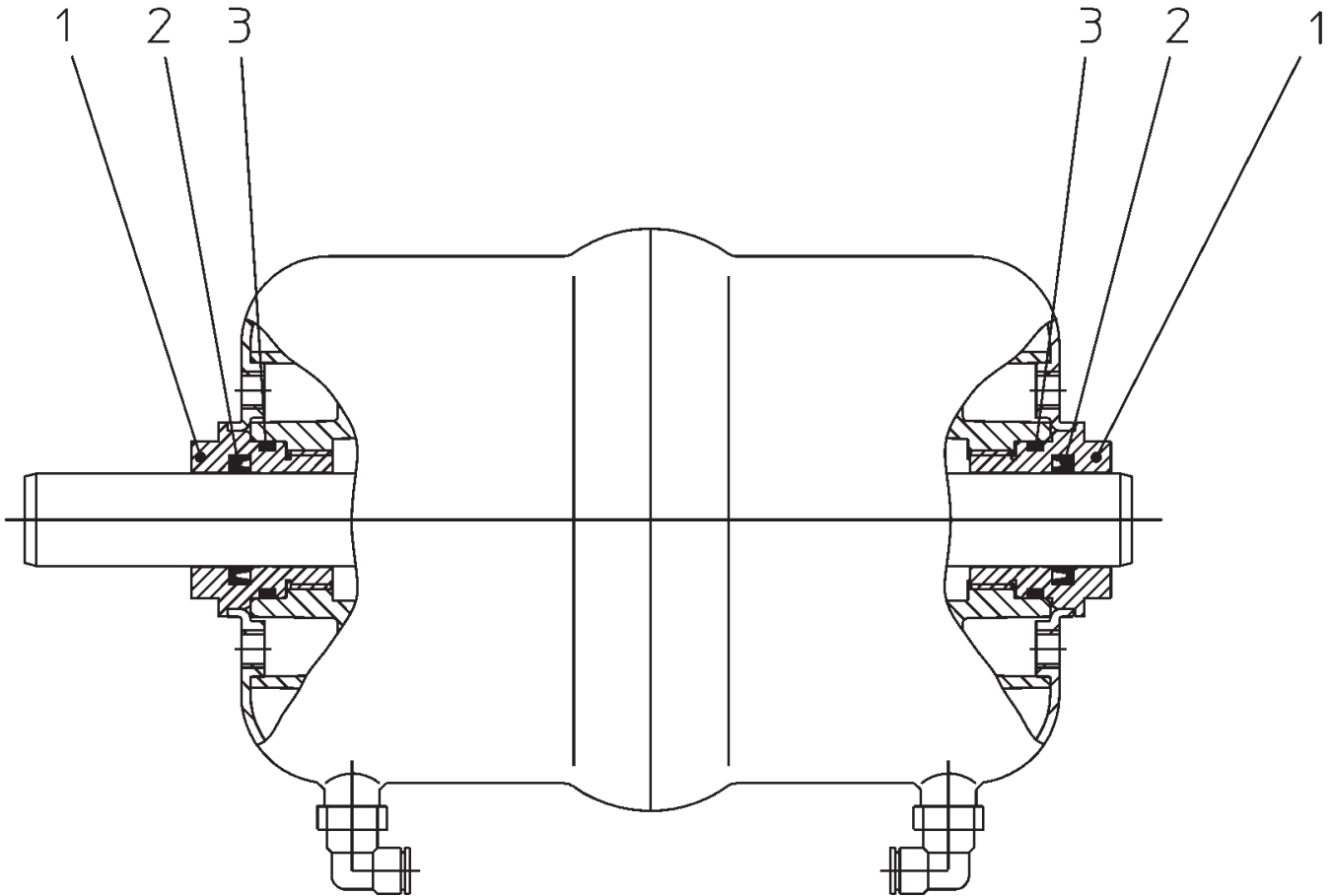
DELTA M4 DIAPHRAGM VALVE ACTUATOR
